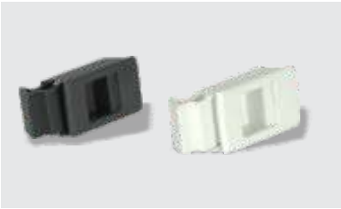
Product Code: FCSL-01 List price: 21.00 Snap Latch Material: Polyamide. Color : Black/Grey.
