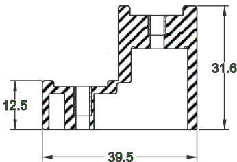
Din Rail Mounted Terminal Base Product Code:- FCNLB-04 Material :- PP FR List Price: 9.50
