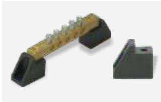
Terminal Base - Height-19mm Product Code FCNLBD-02-DMC FCNLBP-02-Polyamide FCNLBB-02-Bakalite Material :- DMC/Bakalite/Polyamide. List Price:9.50
